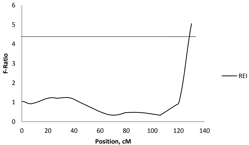
Figure 3.3 Test-statistic along SSC4 for evidence of QTL for residual energy intake (REI) at the growth period of 90 to 120 kg body weight. The solid horizontal line denotes the 95% chromosome-wide significance level.
