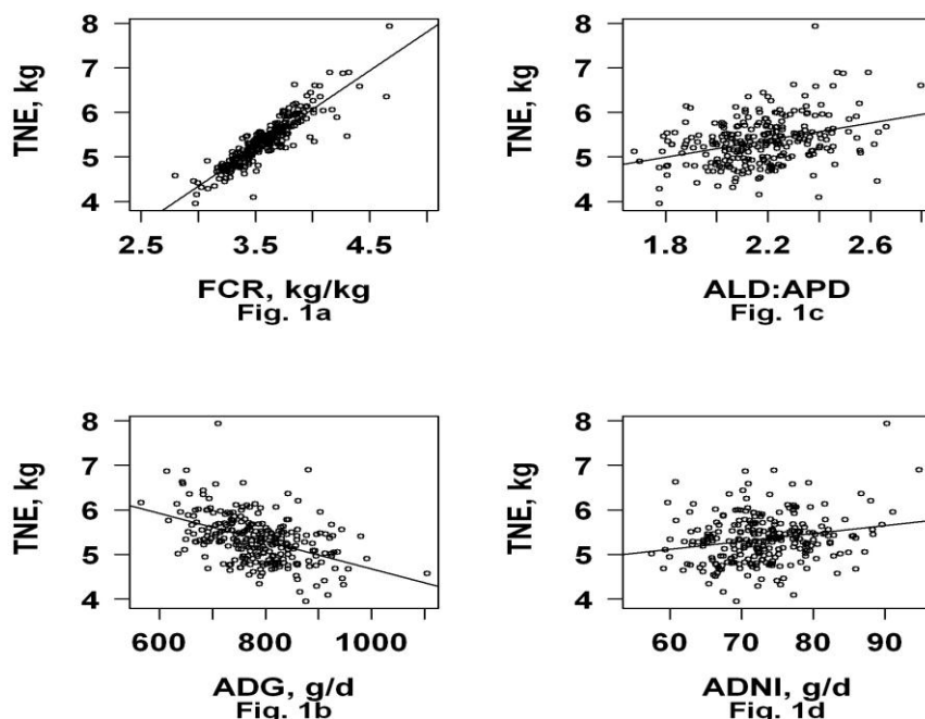
Figure 2.1a-d. Associations between total nitrogen excretion (TNE) and 1a) feed conversion ratio (FCR), 1b) ADG, 1c) lipid to protein gain ratio (ALD:APD), and 1d) average daily nitrogen intake (ADNI) during the entire growing period from 60 to 140 kg.
