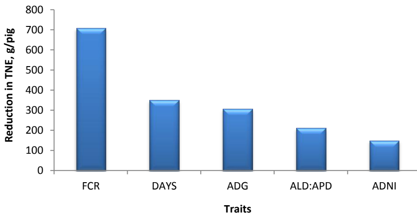
Figure 6.1 Effect of improving feed conversion ratio (FCR), length of growing period (DAYS), average daily gain (ADG), lipid to protein gain ratio (ALD:APD) and average daily nitrogen intake (ADNI) by one standard deviation on total nitrogen excretion (TNE) per pig during the entire growing period from 60 to 140 kg BW
