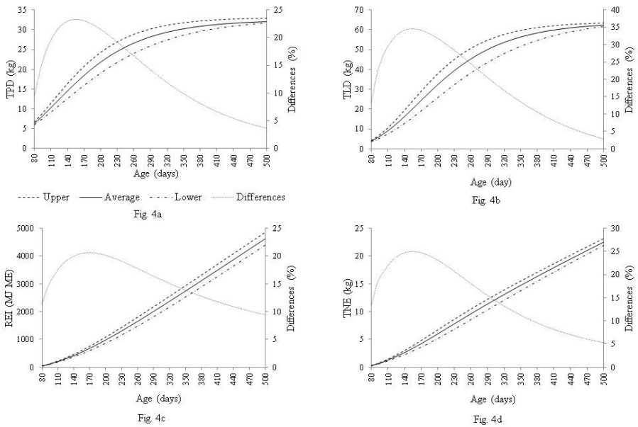
Figure 5.4a-d Growth patterns of total protein weight (TPD), lipid weight (TLD), residual energy intake (REI) and nitrogen excretion (TNE) from 80 to 500 days of age for the entire population (Average) and for selected populations which were at least 1 standard deviation below (Lower) or above (Upper) the average ADG from 30 to 100 kg body weight. The proportional differences between upper and lower category pigs in each 10 day interval are presented as percentages.
