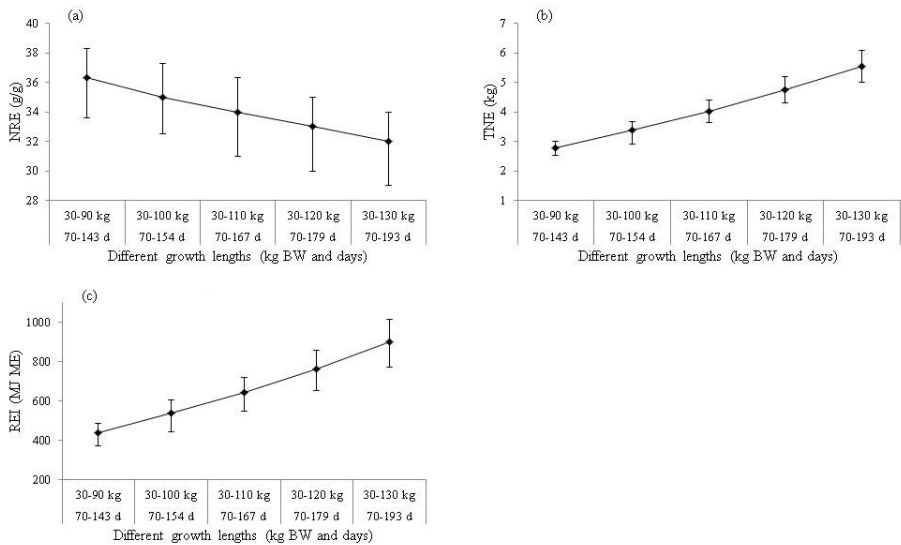
Figure 5.5a-c Average nitrogen retention efficiency (NRE), total nitrogen excretion (TNE) and residual energy intake (REI) at different growth lengths from 30 to 90, 100, 110, 120 and 130 kg slaughter weight, and their respective days of growth for the crossbred population. The upper and lower error bars in NRE represent the estimated trait value for pigs with more than 1 standard deviation above the average ADG at the respective body weight and at least 1 standard deviation below the average ADG at respective body weight, respectively, and vice versa for TNE and REI traits.
