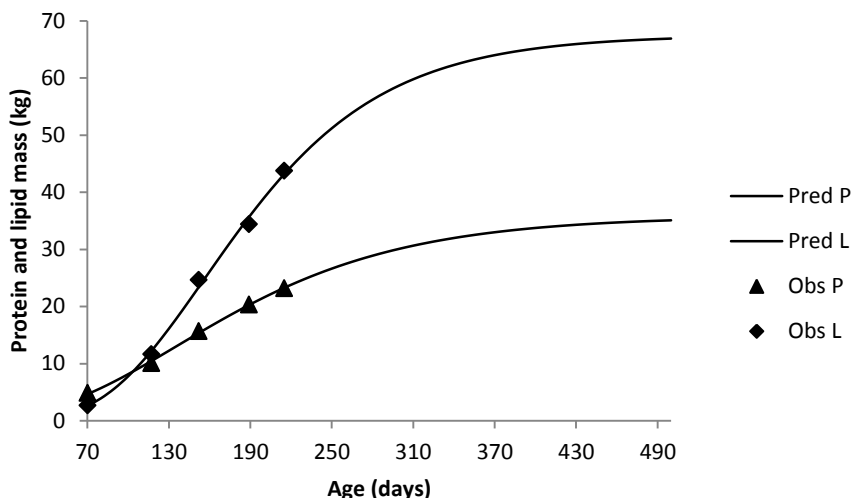
Figure 5.1 Predicted protein (Pred P) and lipid (Pred L) mass by fitting Gompertz curves to observed average protein (Obs P) and lipid (Obs L) mass for one individual pig of the 195 pigs analysed.
