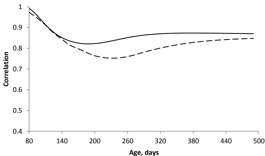
Figure 5.2 Correlations between protein (solid line) and lipid (dash line) mass during growth of pigs from 80 to 500 days of age predicted from the mechanistic biological growth model with the optimal values for the model input parameters and the corresponding estimated values obtained from fitting Gompertz curves through available data (n=195)
