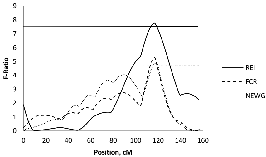
Figure 3.4 Test-statistic along SSC7 for evidence of QTL for residual energy intake (REI), feed conversion ratio (FCR) and nitrogen excretion per weight gain (NEWG) at the growth period of 90 to 120 kg body weight. The solid horizontal line denotes the 95% chromosome-wide significance level for additive QTL for REI, and the dashed horizontal line denotes the 90% chromosome-wide significance level for dominance QTL for FCR and NEWG.
