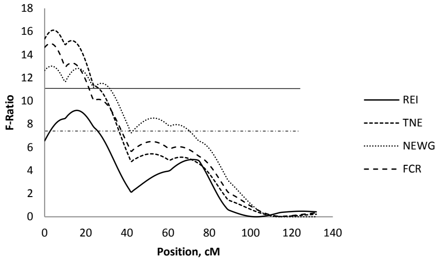
Figure 3.2 Test-statistic along SSC2 for evidence of QTL for residual energy intake (REI), total nitrogen excretion (TNE), nitrogen excretion per weight gain (NEWG) and feed conversion ratio (FCR) at the growth from 90 to 120 kg body weight. The solid and dashed horizontal lines denote the 99% and 95% chromosome-wide significance level, respectively.
