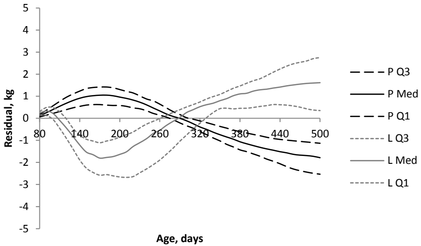
Figure 5.3 Residual estimates for protein and lipid mass during growth of pigs from 80 to 500 days of age predicted from the mechanistic biological growth model with the optimal values for the model input parameters and the corresponding estimated values obtained from fitting Gompertz curves to available data. The median residual for protein and lipid mass (P Med and L Med, respectively) along with third quartile (P Q3 and L Q3, respectively) and first quartile (P Q1 and L Q1, respectively) are presented. Positive values correspond to over-prediction of the mechanistic biological growth model.
