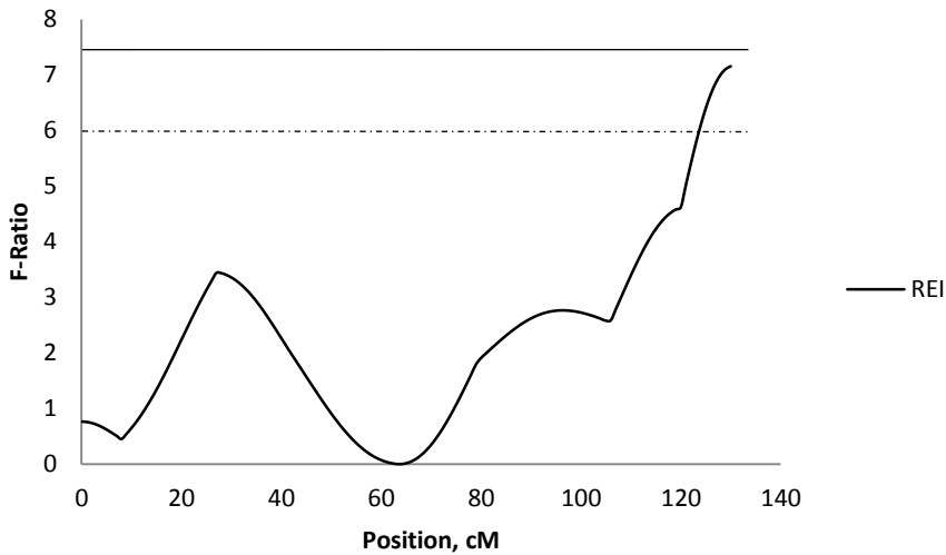
Figure 3.6 Test-statistic along SSC4 for evidence of QTL for residual energy intake (REI) for the entire analysed growth period (60 to 140 kg body weight). The solid and dashed horizontal lines denote the 95% and 90% chromosome-wide significance level, respectively.
