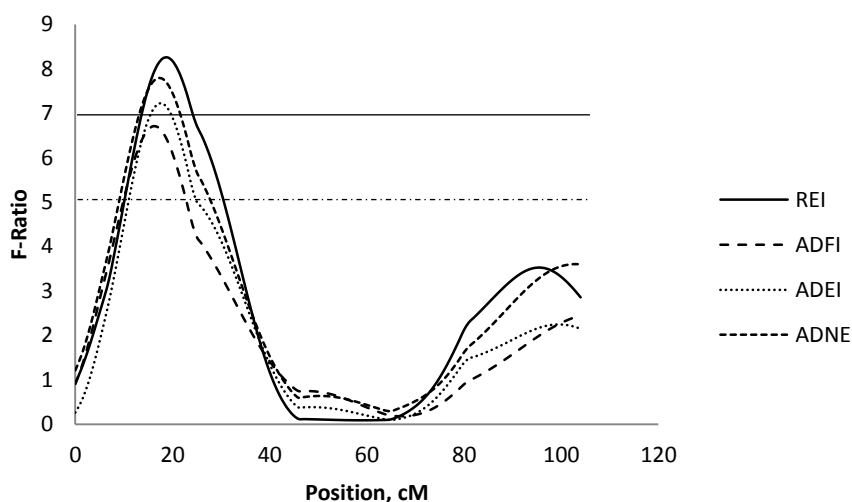
Figure 3.1 Test-statistic along SSC14 for evidence of QTL for residual energy intake (REI), average daily feed intake (ADFI), average daily energy intake (ADEI) and average daily nitrogen excretion (ADNE) at the growth period of 60 to 90 kg body weight. The solid and dashed horizontal lines denote the 99% and 95% chromosome-wide significance level, respectively.
