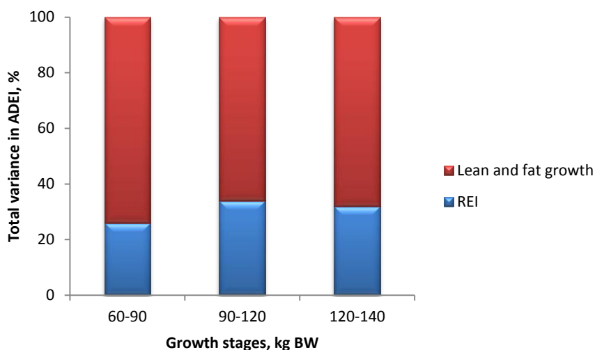
Figure 6.2 Proportion of phenotypic variance in average daily feed intake (ADFI) contributed by residual energy intake (REI) and component traits of REI model (lean and fat growth) at different stages of growth.
