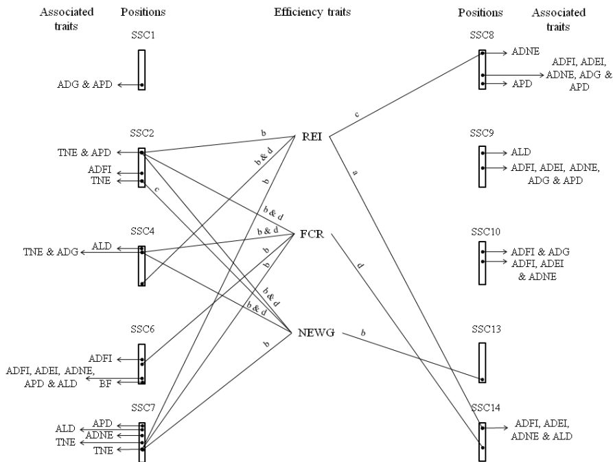
Figure 3.7 The genomic architecture of feed and nitrogen efficiency in association with growth, feed intake and nitrogen excretion traits are presented using QTL information for residual energy intake (REI), feed conversion ratio (FCR), nitrogen excretion per weight gain (NEWG), total nitrogen excretion (TNE), average daily nitrogen excretion (ADNE), average daily feed intake (ADFI), average daily energy intake (ADEI), average daily gain (ADG), average daily protein deposition (APD) and average daily lipid deposition (ALD). The a, b, c and d represent 60 to 90 kg, 90 to 120 kg, 120 to 140 kg growth stages and the entire analysed growth period (60 to 140 kg), respectively.
